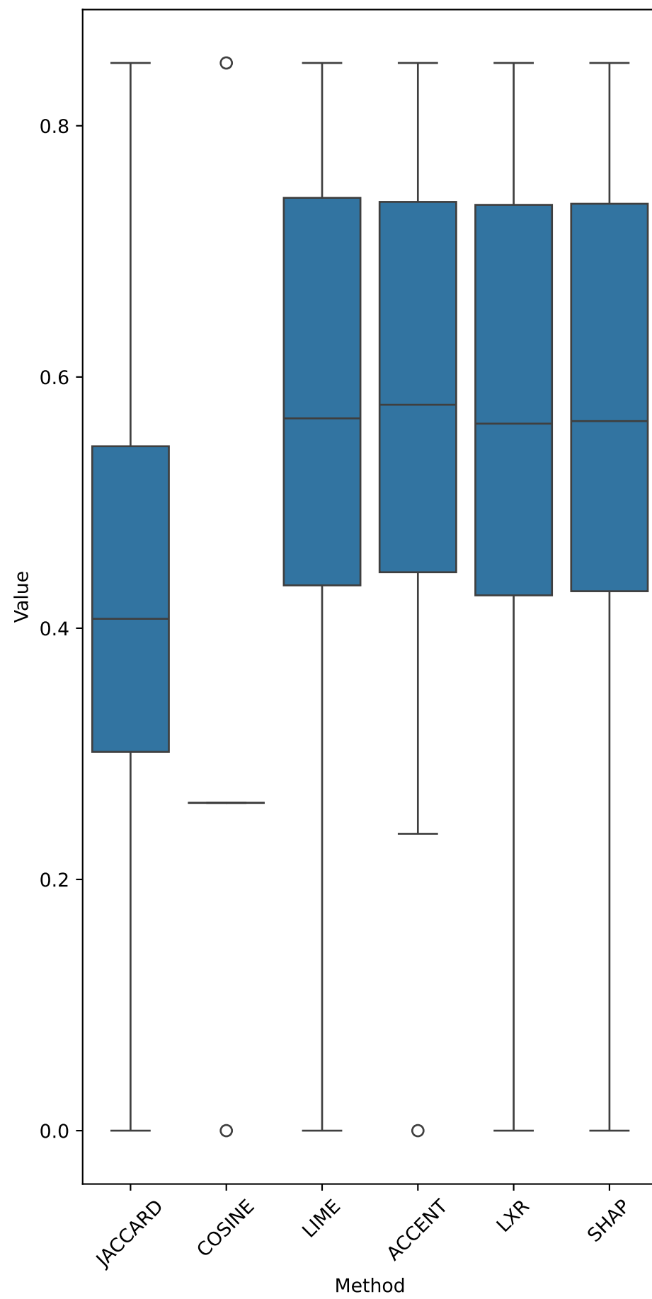
DEL Distribution
