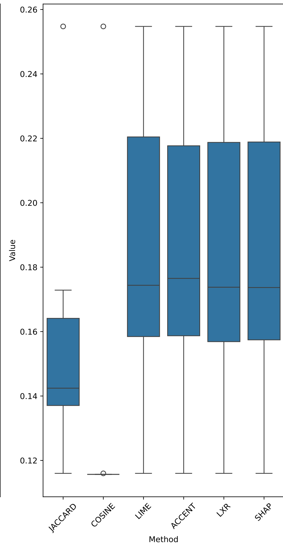
NDCG Distribution
